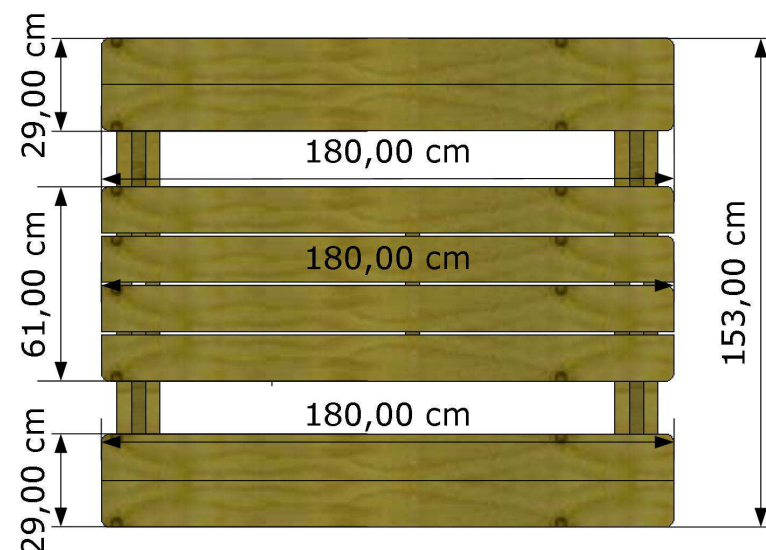
cm. 180x153 – section wood mm. 40
