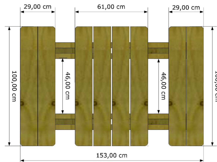
cm. 100x153 – section wood mm. 40
