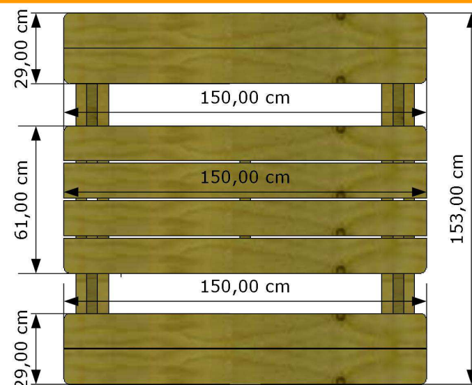
cm. 150x153 - section wood mm. 40
